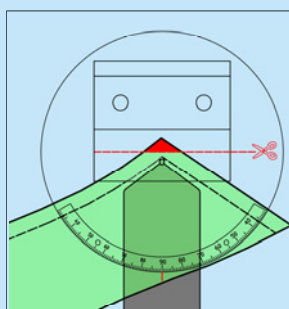
切領－第二刀 Collar trimming – 2 nd cutting
