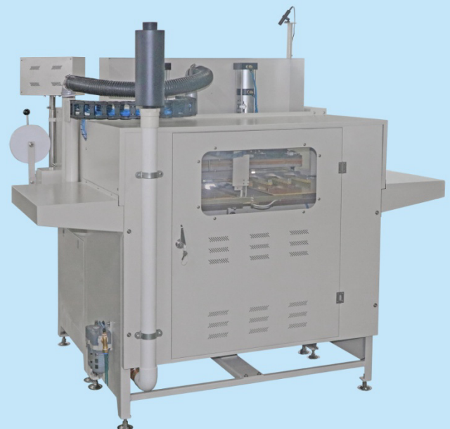
NS-5502 / NS-5502-B 選購平放收料系統 NS-5502 / NS-5502-B Optional horizontal material collecting system
