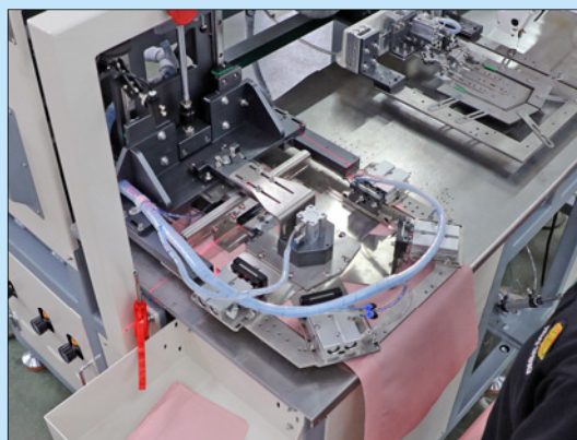
2.機器自動折袋 Automatic pocket folding by machine
