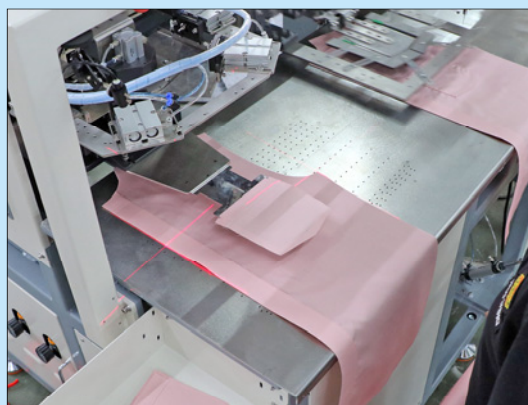
1.擺放口袋裁片(免燙) Laying the cut piece of pocket(iron-free)
