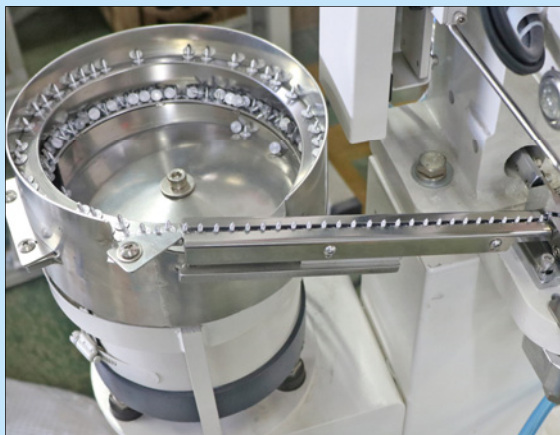
振動鈕扣輸送系統 Vibration Button Feeding System
