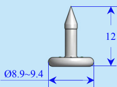
單針鋁鉚釘 Single-pin aluminum rivet
