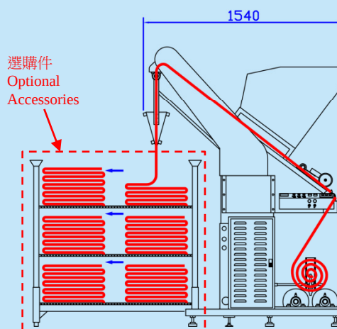
O-A-12-01 三層放布架 O-A-12-01 3-layer fabric stand
