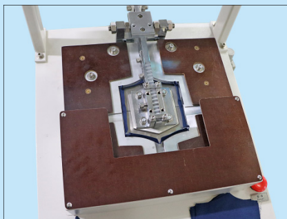
袋蓋模四邊同時摺熨 Pocket flap mould creases all sides
