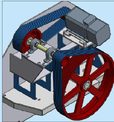
兩級皮帶傳動 Two-stage belt transmission
