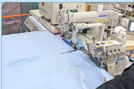
釁骨和間線二合一操作 Integrated process of overlocking and topstitching
