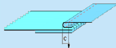
2.平車自動間線(C=1~5mm) topstitching by lockstitch machine (C=1~5mm)
