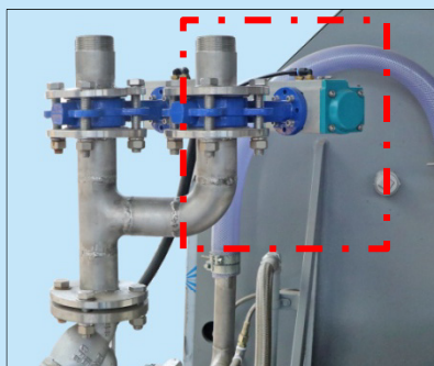
O-I-04-2-1 電控氣動入水系統-Ø2" Electric Controlled Water Feeding System -Ø2"
