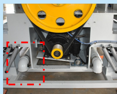
O-I-28-01-04 另增氣動排水控制系統-Ø4" Additional Pneumatic Water Draining Control System -Ø4"
