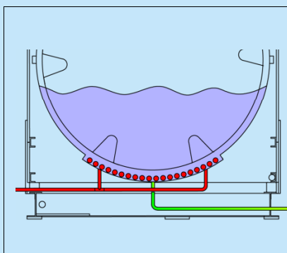
O-I-63-07 間接保溫系統-內部 Indirect insulation system-Internal
