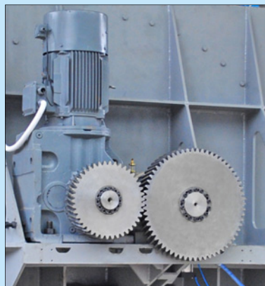
齒輪驅動系統 Gear driving system
