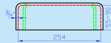
圓角袖口模 Round corner cuff template
