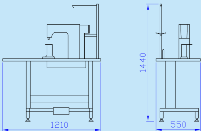
側骨間線操作 Side seam topstitch operation
