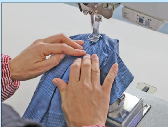
側骨間線操作 Side seam topstitch operation
