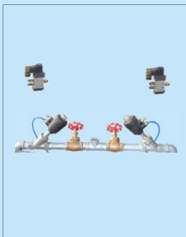
蒸汽(直接/間接加溫)氣動閥總成- Ø1" (NS-2713) Steam (Direct/Indirect Heating) Pneumatic Valve Assy-Ø1" (NS-2713)
