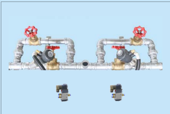
蒸汽(直接/間接加溫)氣動閥總成-Ø1" (NS-2701) Steam (Direct/Indirect Heating) Pneumatic Valve Assy-Ø1" (NS-2701)
