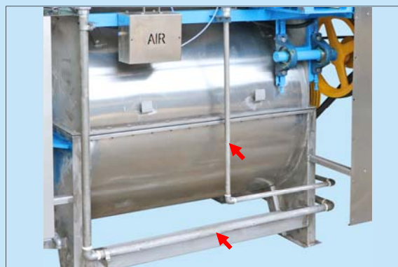
蒸汽直接加溫與間接加溫裝置(NS-2701-70~100) Direct and indirect steam heating device(NS-2701-70~100)
