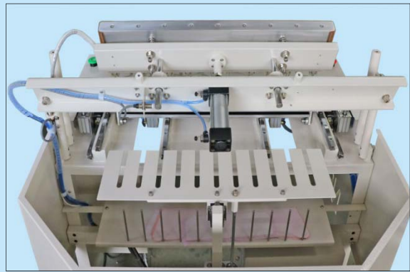
快速翻轉上模清潔設計 Quick flipping upper mould for cleaning design
