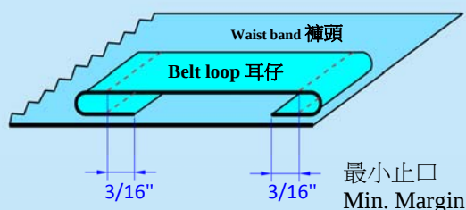
耳仔成品示意圖 Schematic Diagram of finished belt loop
