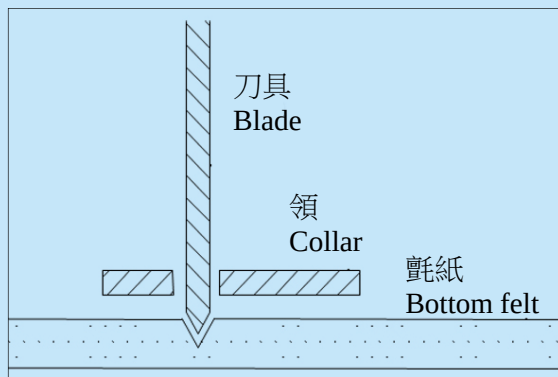
自動移動氈紙，保護刀鋒 Bottom felt sheet can move for blade edge protection
