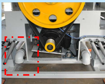
另增氣動排水控制系統 Additional Pneumatic Water Draining Control System
