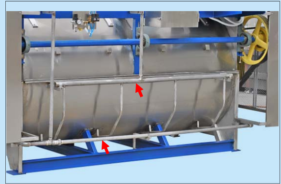
蒸汽直接加溫與間接加溫裝置(NS-2701) Direct and indirect steam heating device(NS-2701)
