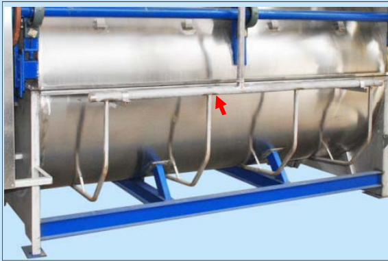
蒸汽直接加溫裝置(NS-2700) Direct steam heating device (NS-2700)
