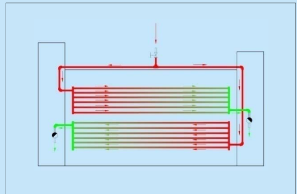
蒸汽間接加溫示意圖(NS-2701) Indirect steam heating diagram (NS-2701)
