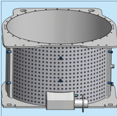
外殼間接保溫系統 Shell indirect heat preservation system
