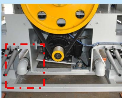
O-I-28-01-04 附加排水系統-Ø4" Optional Water Draining System -Ø4" (suitable for Wassar 220S)
