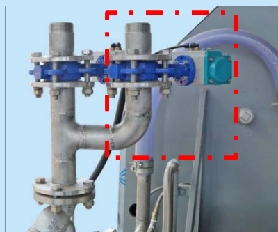
O-I-04-2-1 電控氣動入水系統-Ø2" Electric Controlled Water Feeding System -Ø2" (suitable for Wassar 220S)
