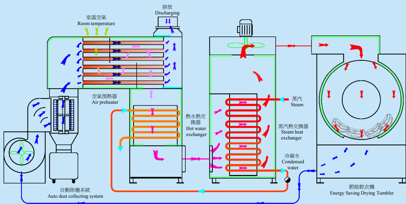
乾衣機工作原理圖 Work principle diagram of drying tumbler
