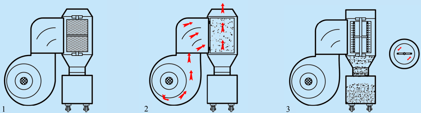
自動環保除塵系統工作原理 Work principle of environment-friendly automatic de-dusting & filtering system
