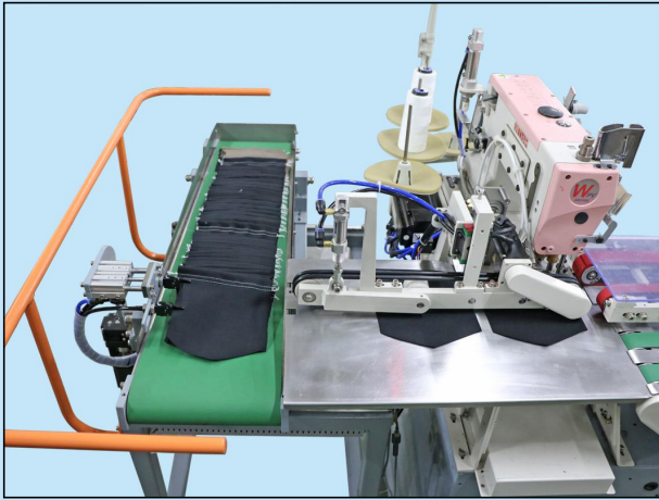
自動縫紉、傳送帶自動收料系統 Automatic sewing, and conveyer belt collecting system
