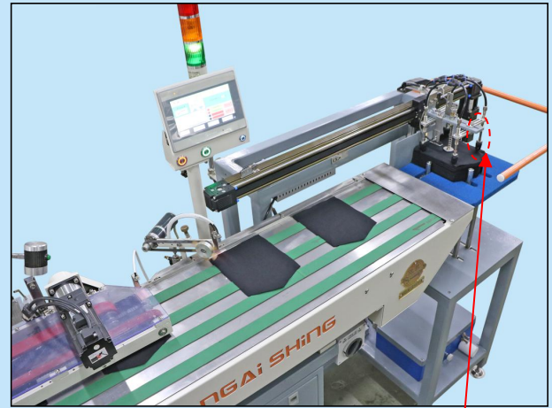
機械手自動上料、輸送、摺邊系統 Robot automatic loading, feeding and folding system
