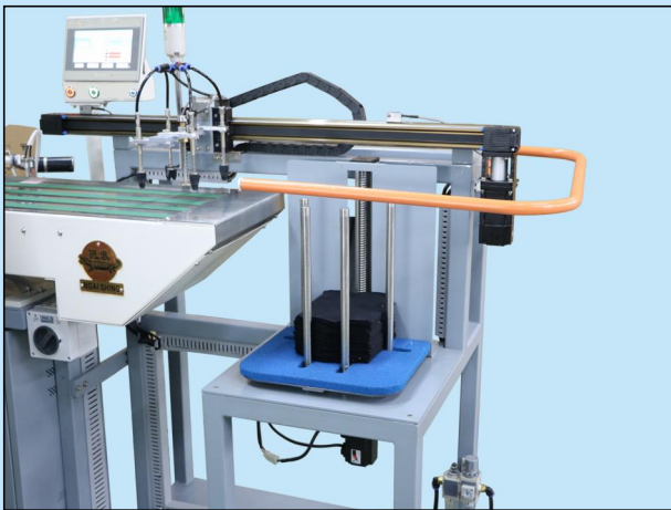
智能物料升降台 Intelligent material lifting platform
